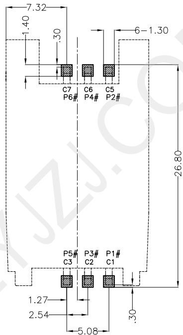
RECOMMENDED PCB PATTERN DIM. TOLERANCE : ±0.05
